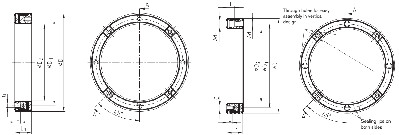
Damping ring type DT (patent pending) and DTV
